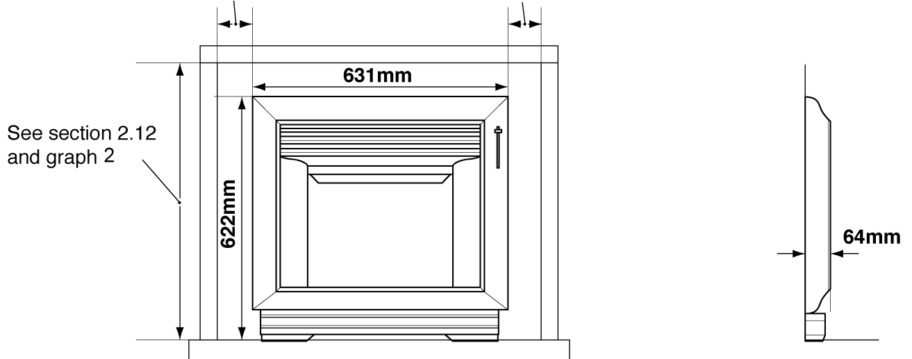
Figure 1 Continued. Appliance dimensions
