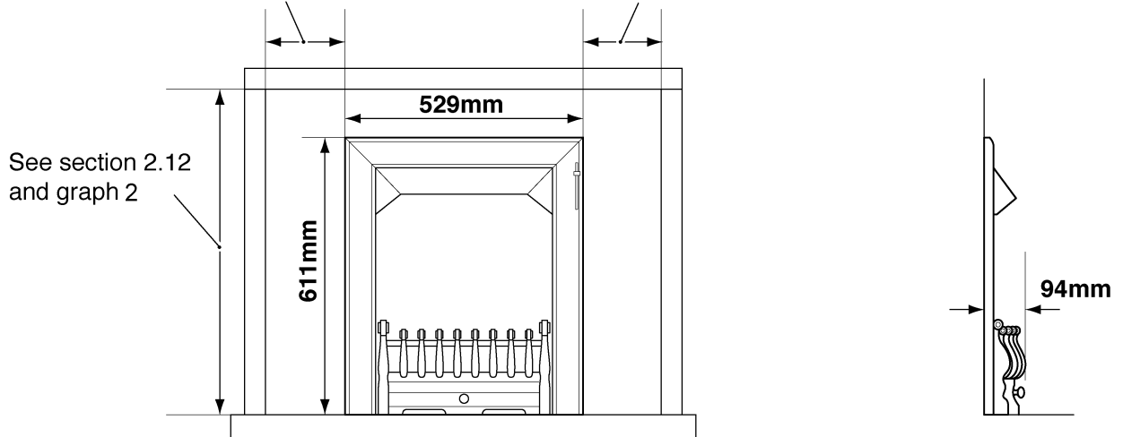
Figure 1. Appliance dimensions (Continued on next page)
