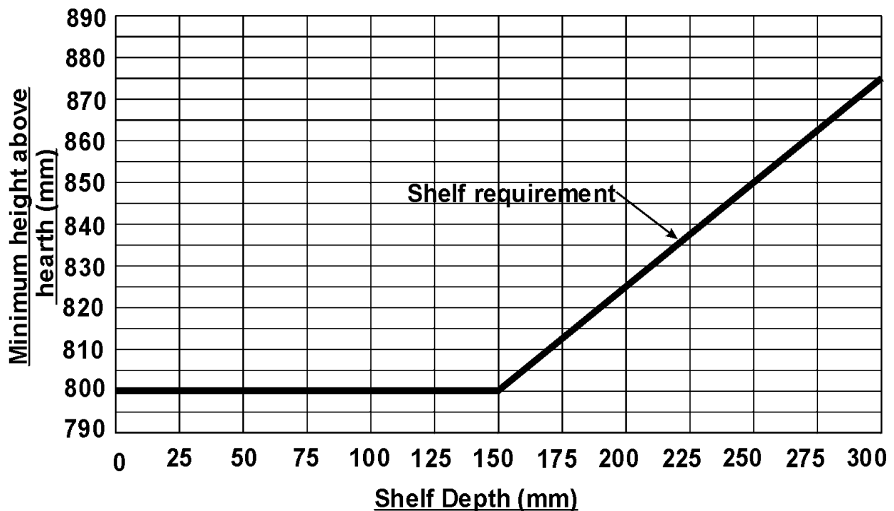
Graph 1. Combustible shelf clearances for ADORN model only
